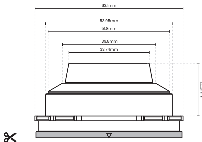
16-30mm T2.9 PL Mount
