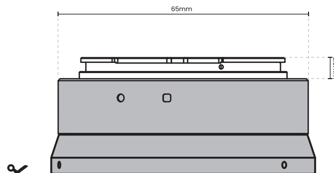
28-75mm T2.9 EF Mount
