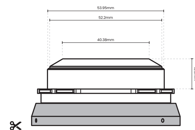
75-180mm T2.9 PL Mount
