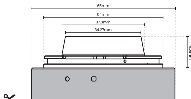
16-30mm T2.9 EF Mount
